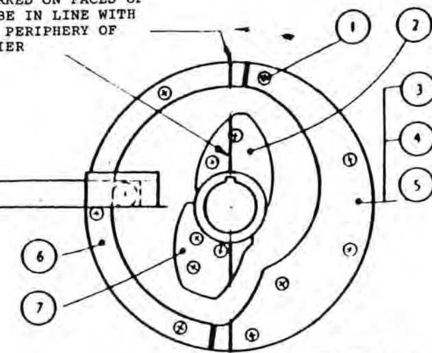
SECTION 587B 6TH POSITION THREADING CAM ACCELERATED TIMING
