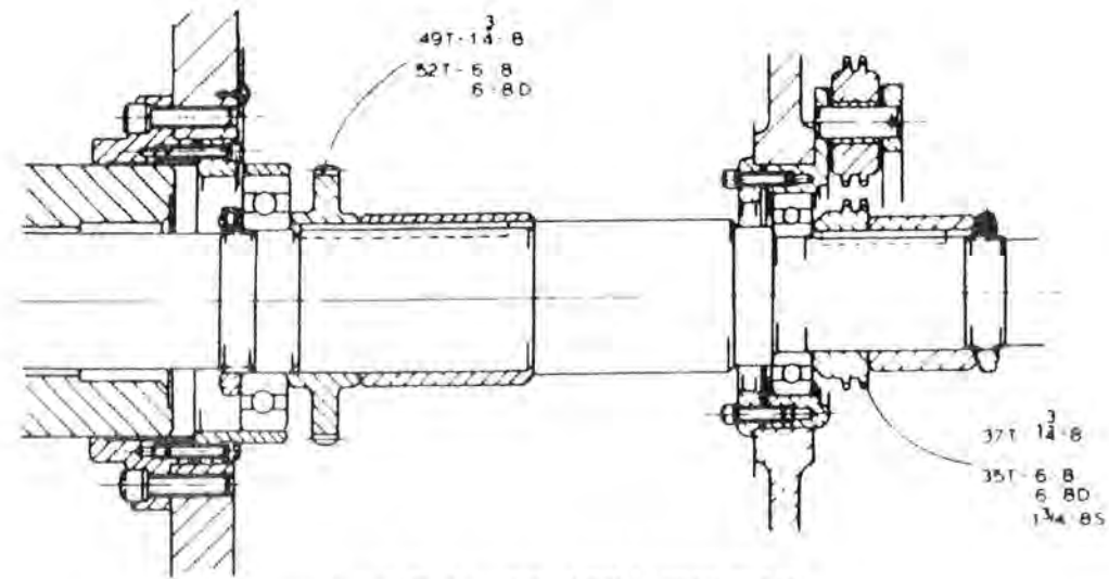
CENTRE SHAFT ARRANGEMENT FOR 1 3/4-8, 6-8 & 6-80
